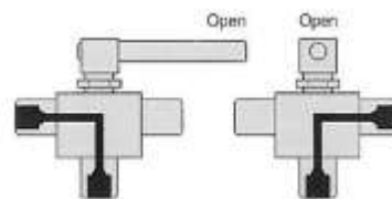
90° Three-Way Diverter Valve
