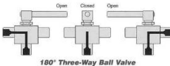
180° Three-Way Ball Valve
